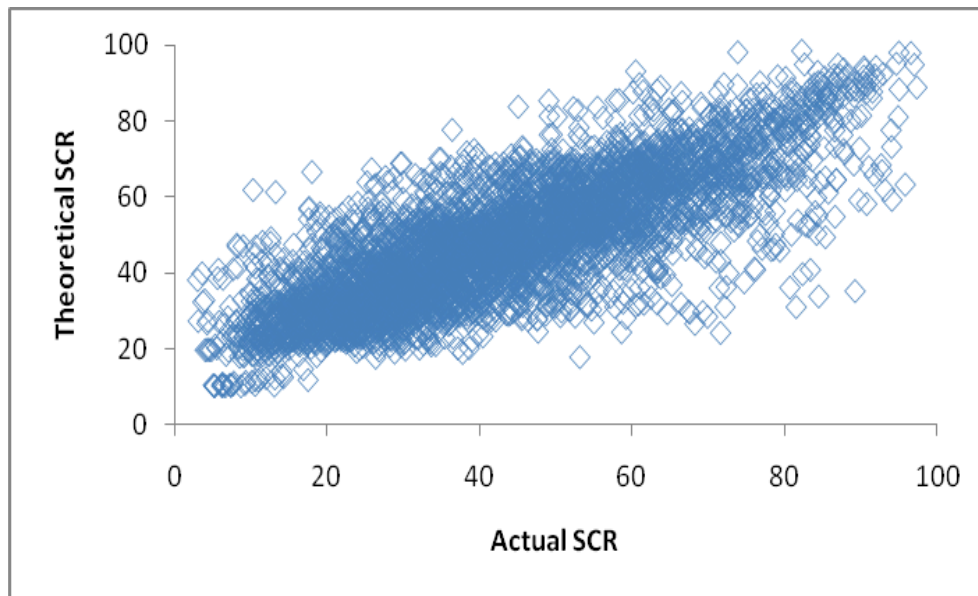
Figure 1: Relationship between Actual and Theoretical SCR ( r = 0.79 )
