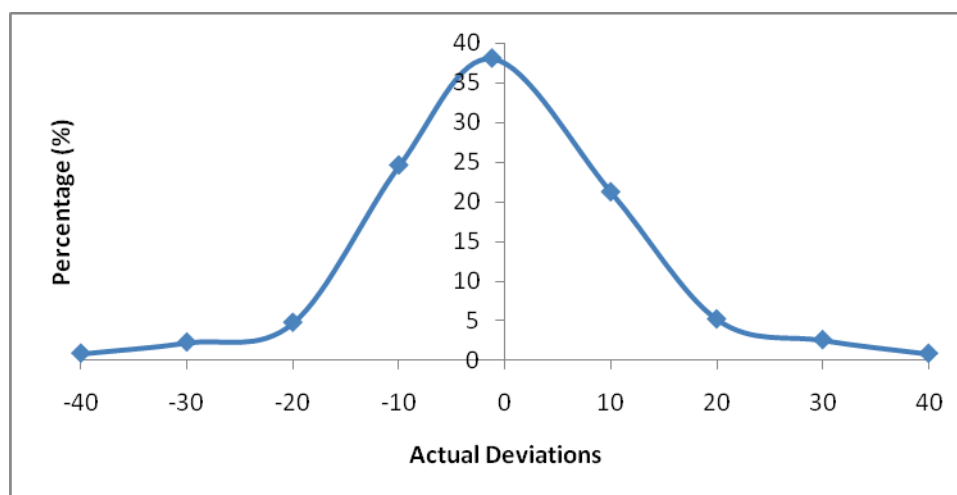
Figure 2: Empirical distribution of SCR Deviations
